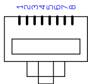
RJ-45 8-pole Plug seen from cable entry
