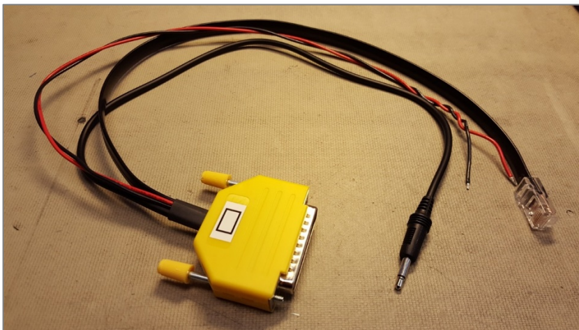
Cable Kit for Icom radios w/o back connector
